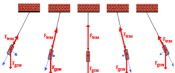
Fig 3.3 the direction of forces along the axis of Pendulum at different positions
