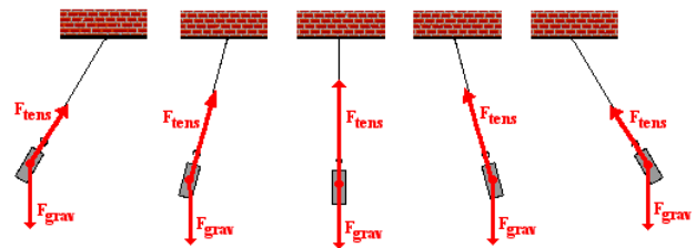
The force of gravity is always directed downward; its magnitude never changes. The tension force is always directed towards the pivot; its magnitude varies over the course of a vibrational cycle.
