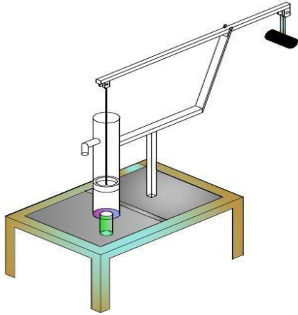
Fig 6.1: 3D Model of Hand Water Pump with Pendulum
