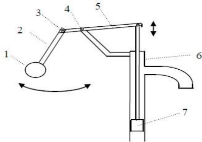
Fig 2.1 Schematic hand water pump with pendulum.
